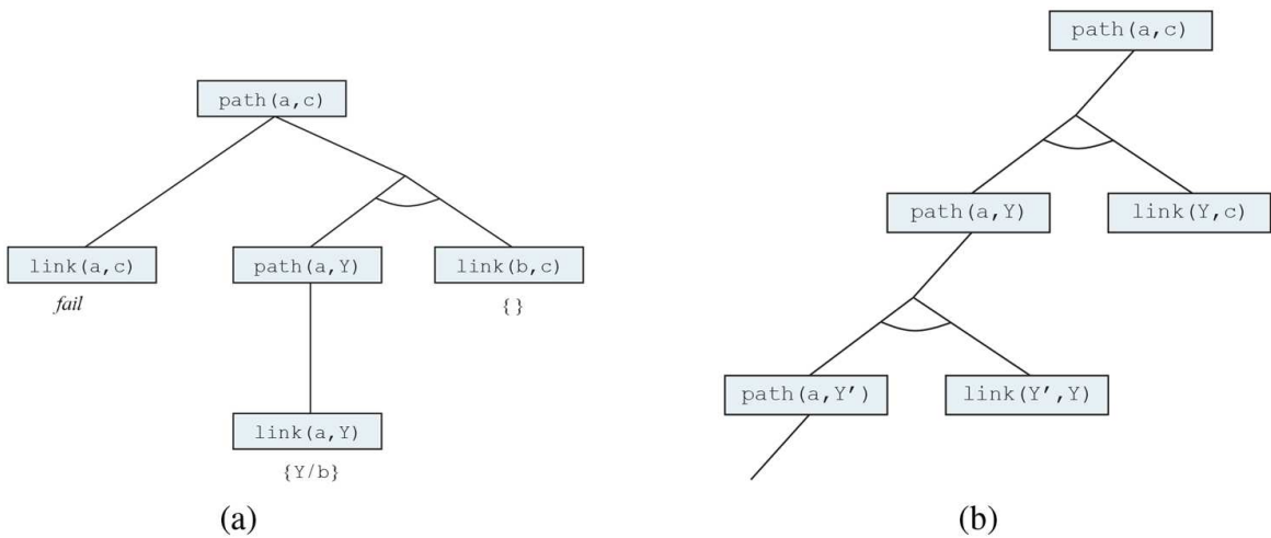
(a) Proof that a path exists from A to C . (b) Infinite proof tree generated when the clauses are in the “wrong” order.
