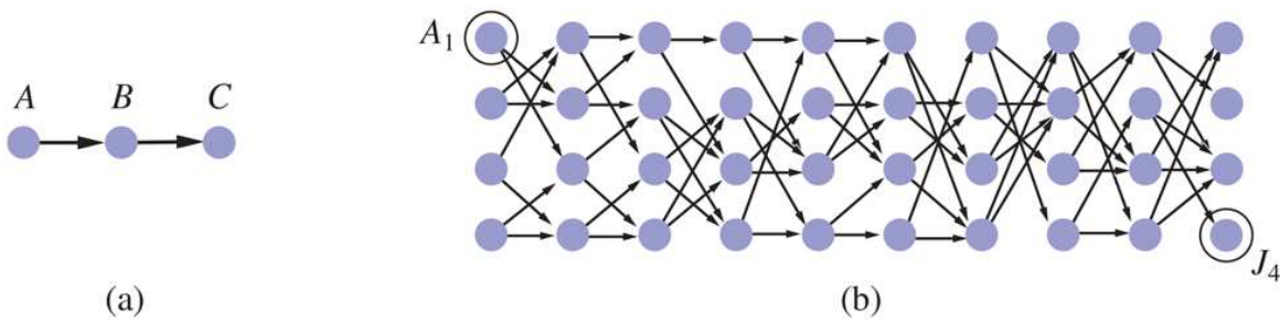
(a) Finding a path from A to C can lead Prolog into an infinite loop. (b) A graph in which each node is connected to two random successors in the next layer. Finding a path from A 1 to J 4 requires 877 inferences.
