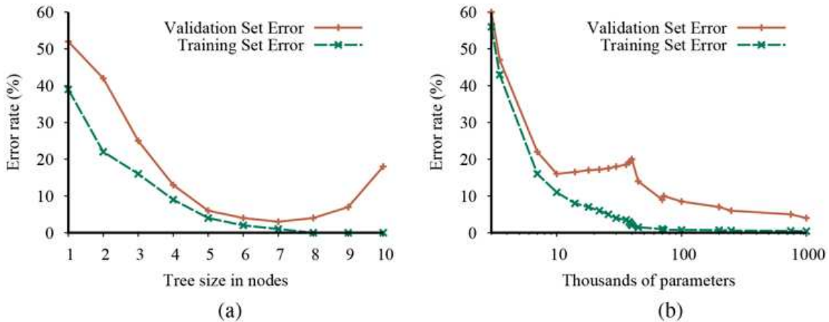
Error rates on training data (lower, green line) and validation data (upper, orange line) for models of different complexity on two different problems. MODEL-SELECTION picks the hyperparameter value with the lowest validation-set error. In (a) the model class is decision trees and the hyperparameter is the number of nodes. The data is from a version of the restaurant problem. The optimal size is 7. In (b) the model class is convolutional neural networks (see Section 21.3) and the hyperparameter is the number of regular parameters in the network. The data is the MNIST data set of images of digits; the task is to identify each digit. The optimal number of parameters is 1,000,000 (note the log scale).
